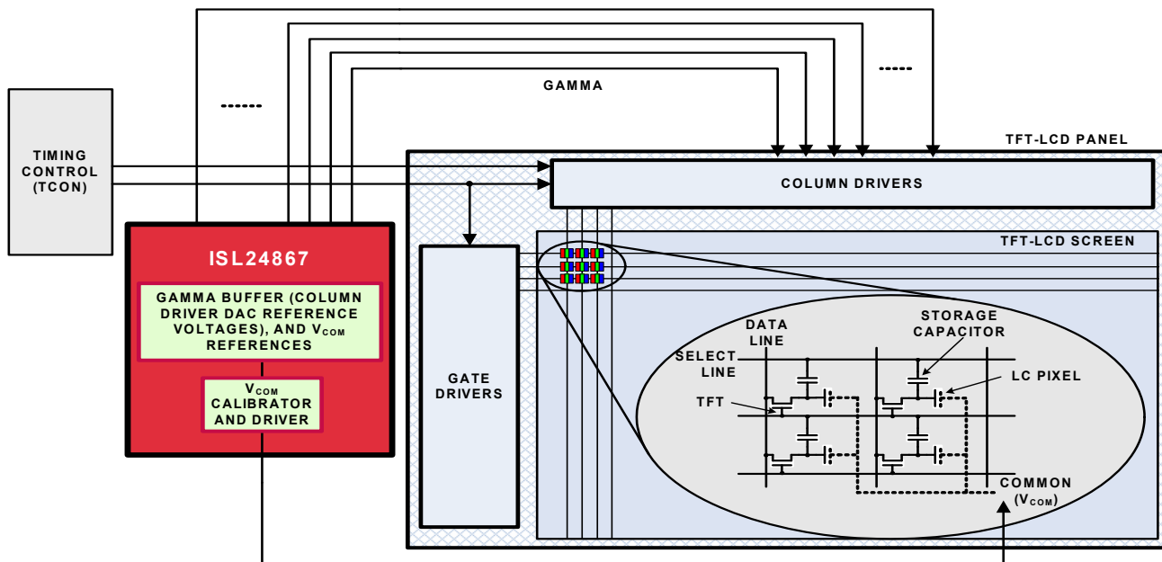
FIGURE 1. TYPICAL APPLICATION: TFT-LCD REFERENCE VOLTAGE GENERATOR
